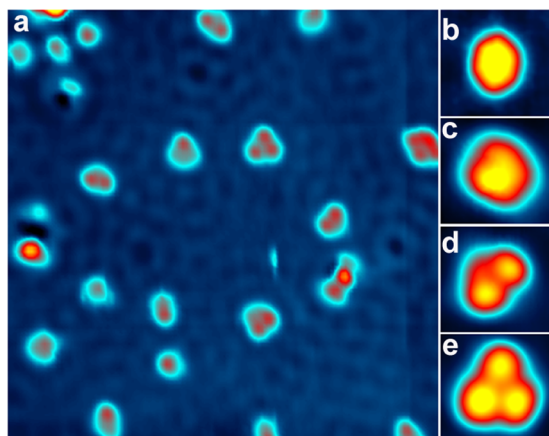
Figure 1. (a) STM image of water clusters on Cu(111) surface. Image size: 20 \times 20 \text{ nm}^2 . Image is taken under sample bias of 20 mV and tunneling current of 10 pA. (b–e) STM images of single water cluster of different sizes: hexamer (b), heptamer (c), octamer (d), and nonamer (e). Image size: 2 \times 2 \text{ nm}^2 .
