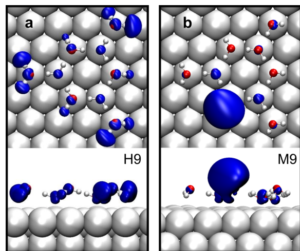
Figure 4. Top and side views of LUMO state in H9 (a) and M9 (b) nonamers on Cu(111) surface.
